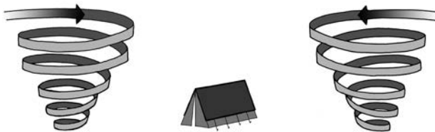
Figure 3: These vortices pass on both sides of the tent and continue down the slope until they dissipate.
