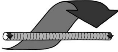
Figure 1: Wind shear is caused by friction with the surface, increasing with height as it travels up the mountain, and rolling up to create a horizontal roll vortex or tornado.
