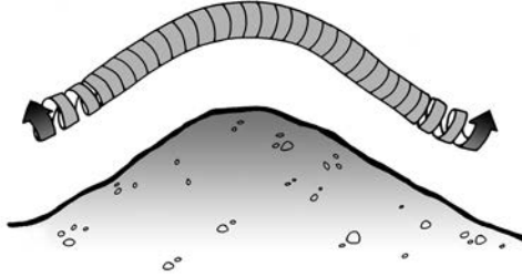
Figure 2: As the horizontal vortex rolls over the dome of the mountain, it is tilted upward and strengthens into a pair of vertical tornadoes or vortices.
